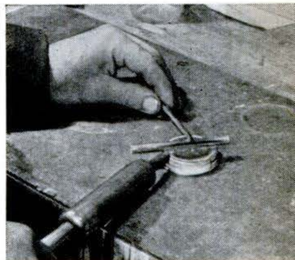
SOLDER tube assembly to cap after aligning punched hole in the cap with drilled hole in the tube.
